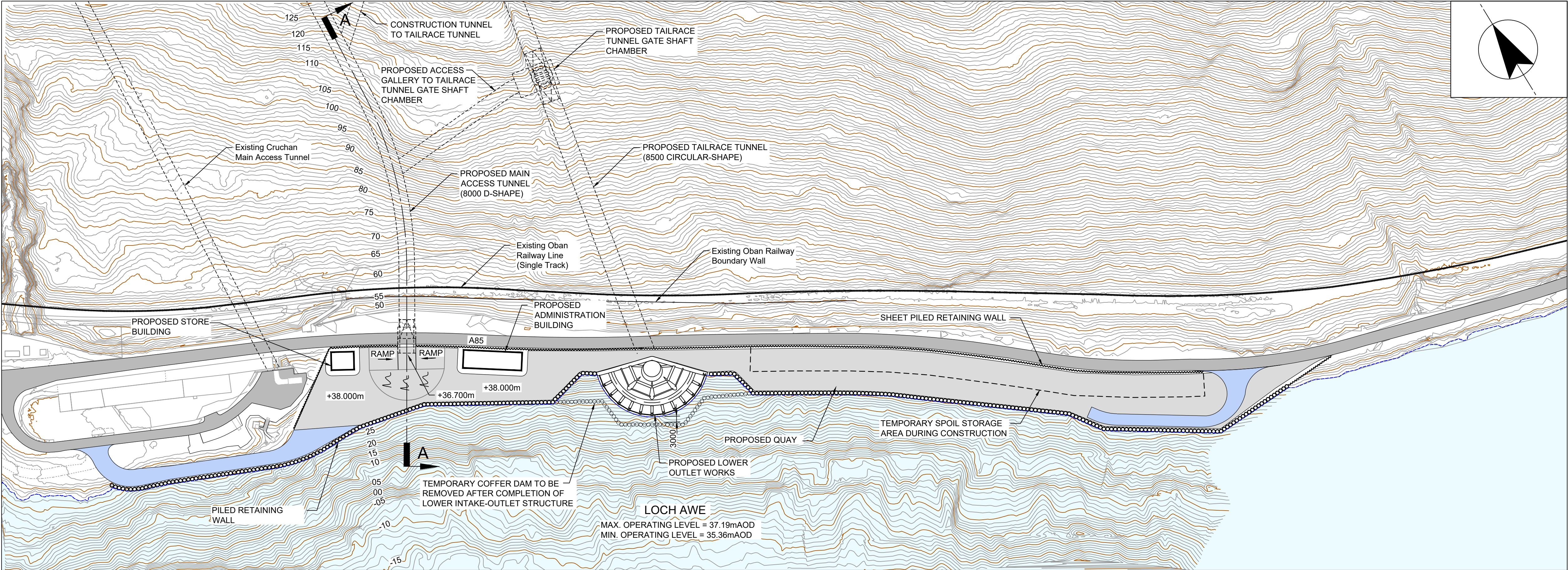
PLAN (SCALE 1: 1250)
